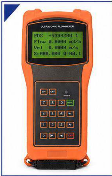
Front Device View
